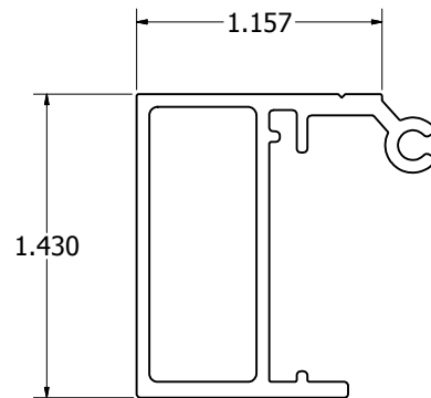
SERIES 7-12 FRAMELESS RETAINER PART# 1631
